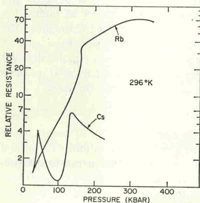
FIGURE 2 (left). Resistance vs pressure—cesium and rubidium.
