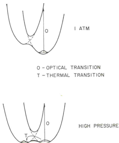
FIGURE 1. Schematic configuration coordinate diagram.
